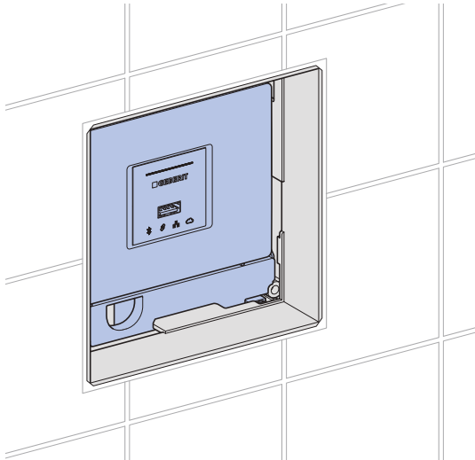
Figure 11: Mounting in installation box
