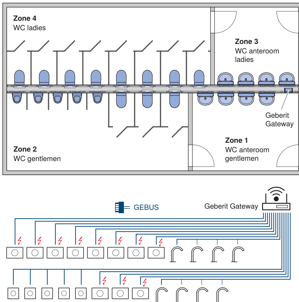
Figure 25: Practical example 1: Connection via GEBUS
