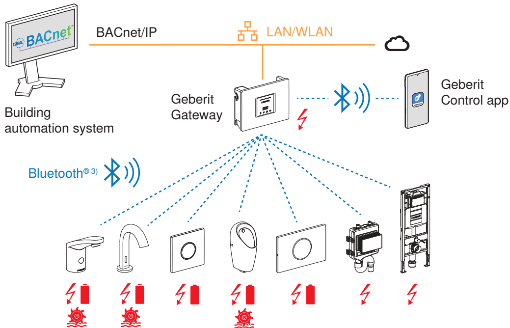
Figure 9: Connection of Geberit Connect end devices via Bluetooth®
