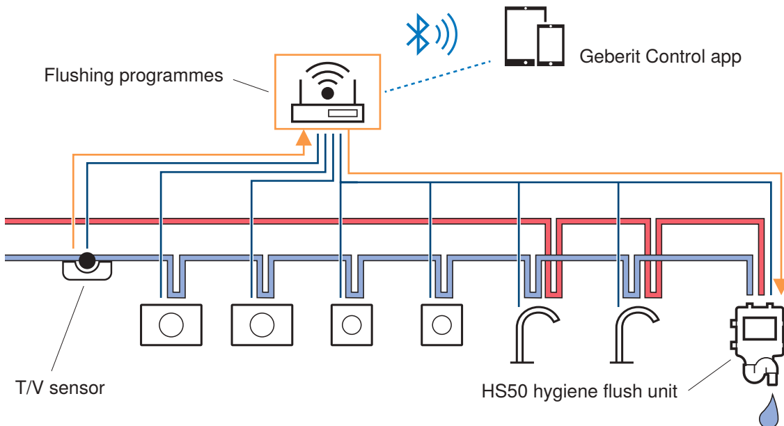
Figure 20: Example: Geberit Gateway with flushing programmes in connected operation
