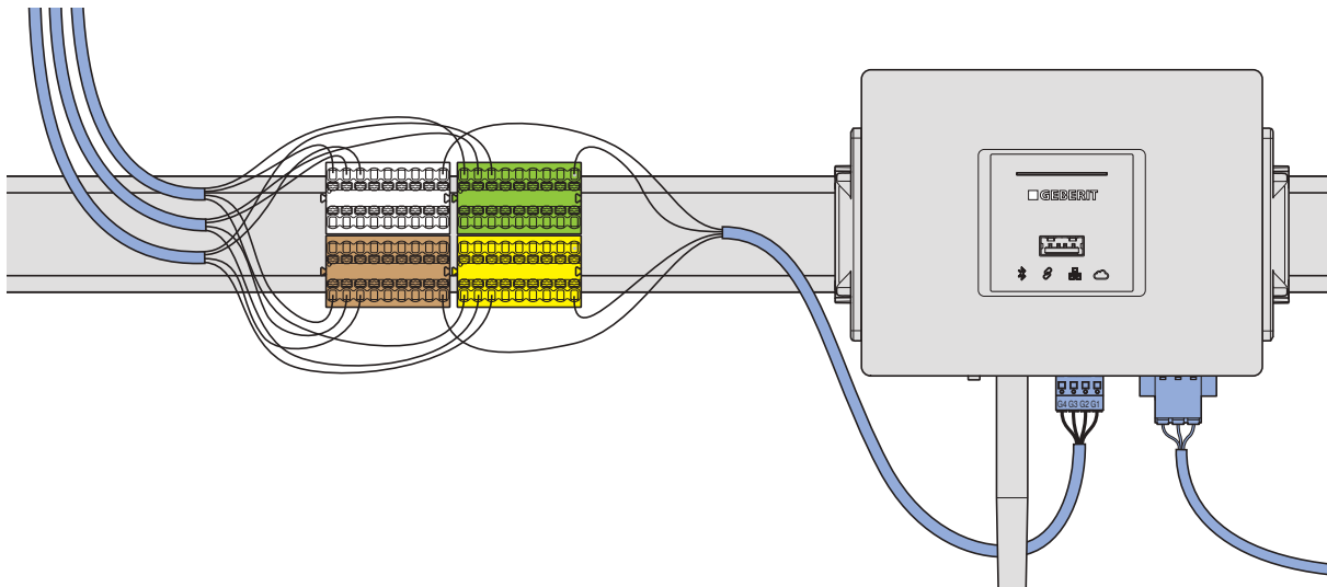
Figure 15: Terminal block for connecting the GEBUS cable
