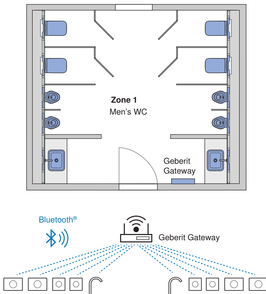
Figure 27: Practical example 2: Connection via Bluetooth®
