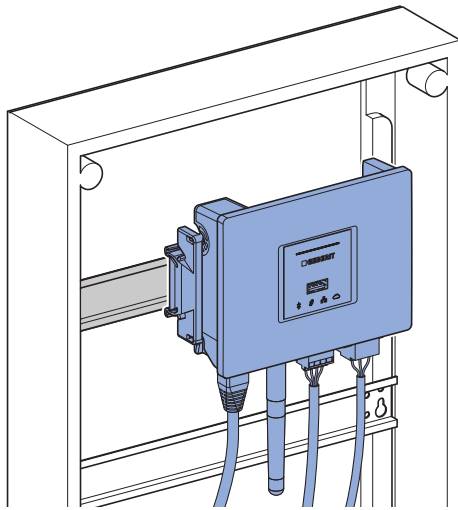
Figure 12: Mounting in the control cabinet
