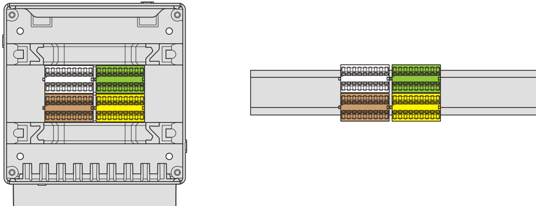
Figure 6: Terminal block in the installation box (left) and mounted on a top-hat rail for control cabinet installation (right)
