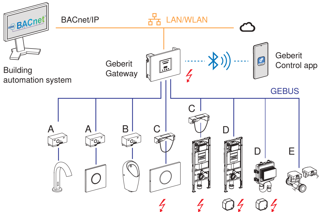
Figure 8: Connection of Geberit Connect end devices via GEBUS
