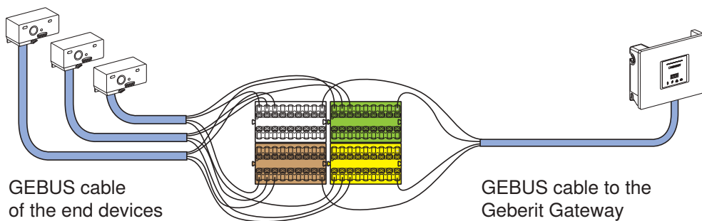
Figure 7: Example for the connection of 3 Geberit Connect end devices with the Geberit Gateway
