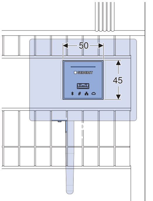
Figure 14: Minimum size of the openings in the control cabinet cover
