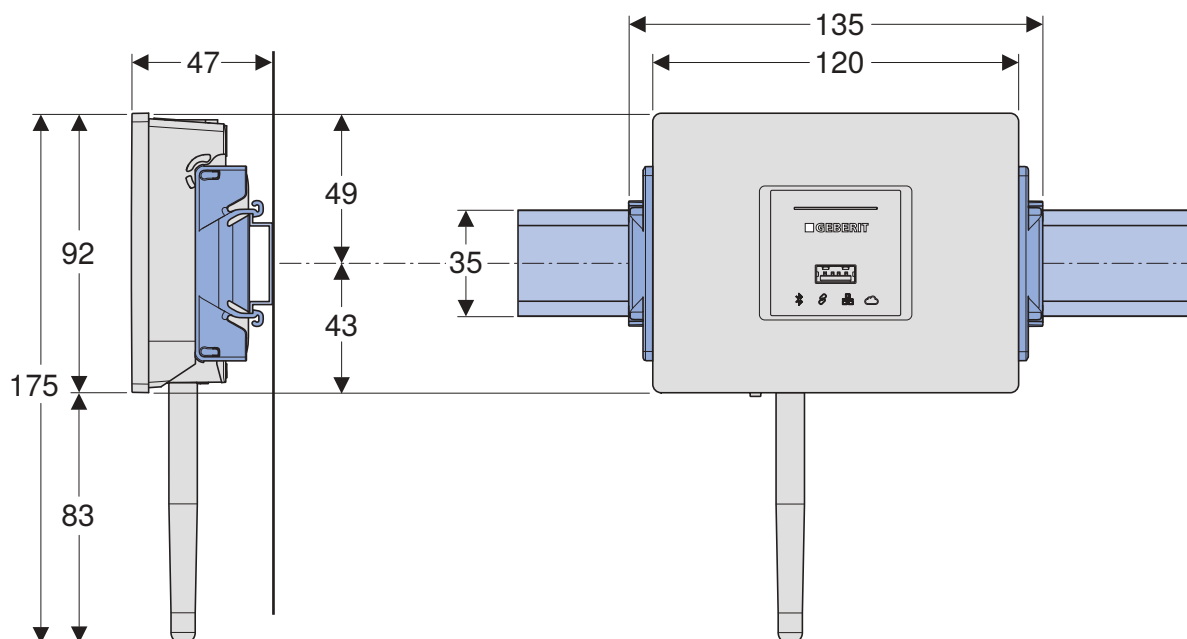
Figure 13: Dimensions for mounting on DIN top-hat rails
